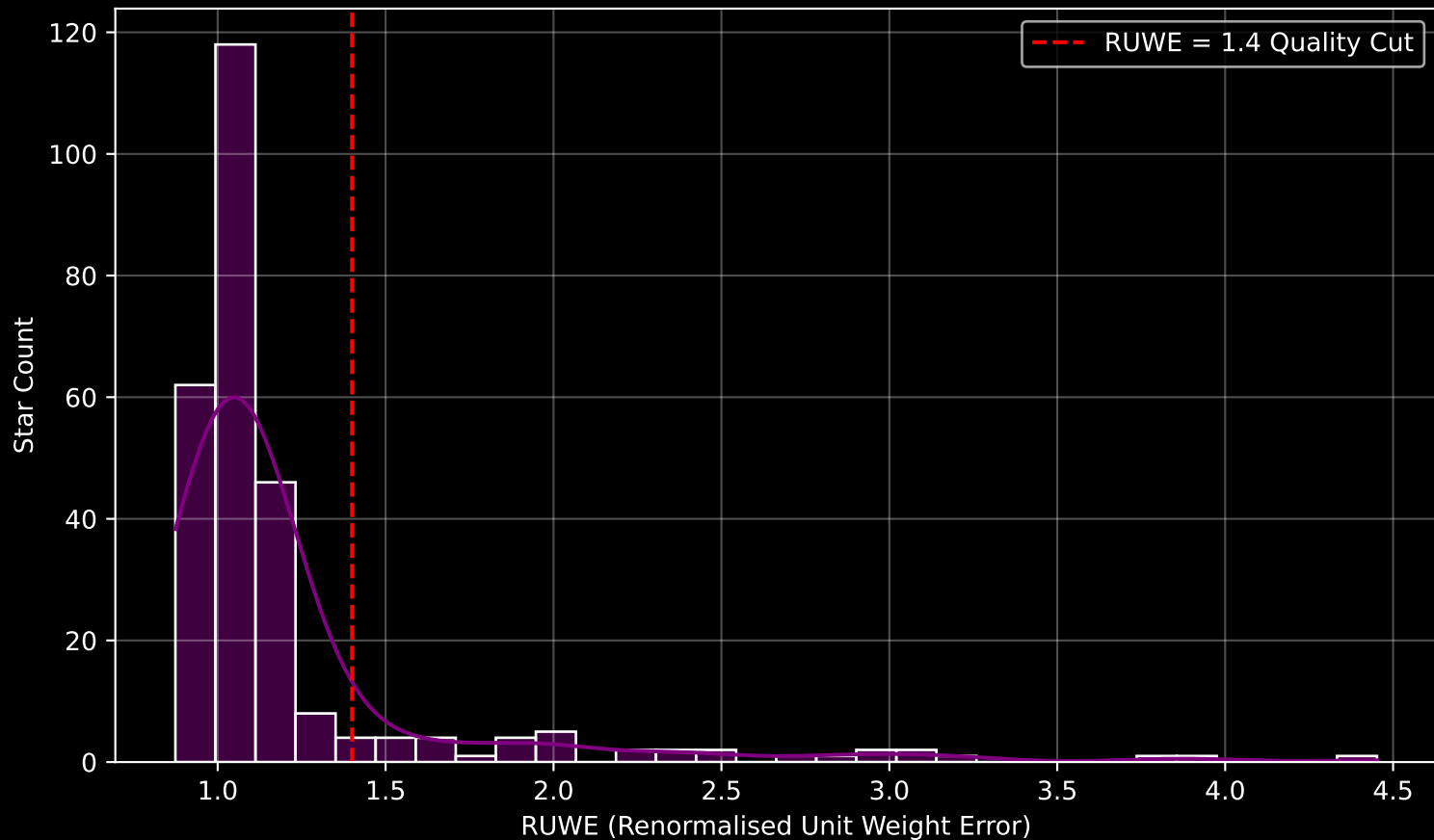
GALAH DR4 Field [237] RUWE Distribution (n= 272)
