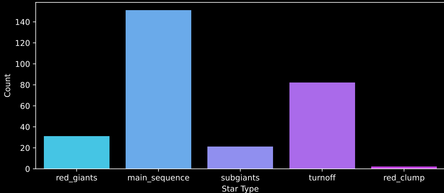
GALAH DR4 Field: [237] Count plot of Star Type
