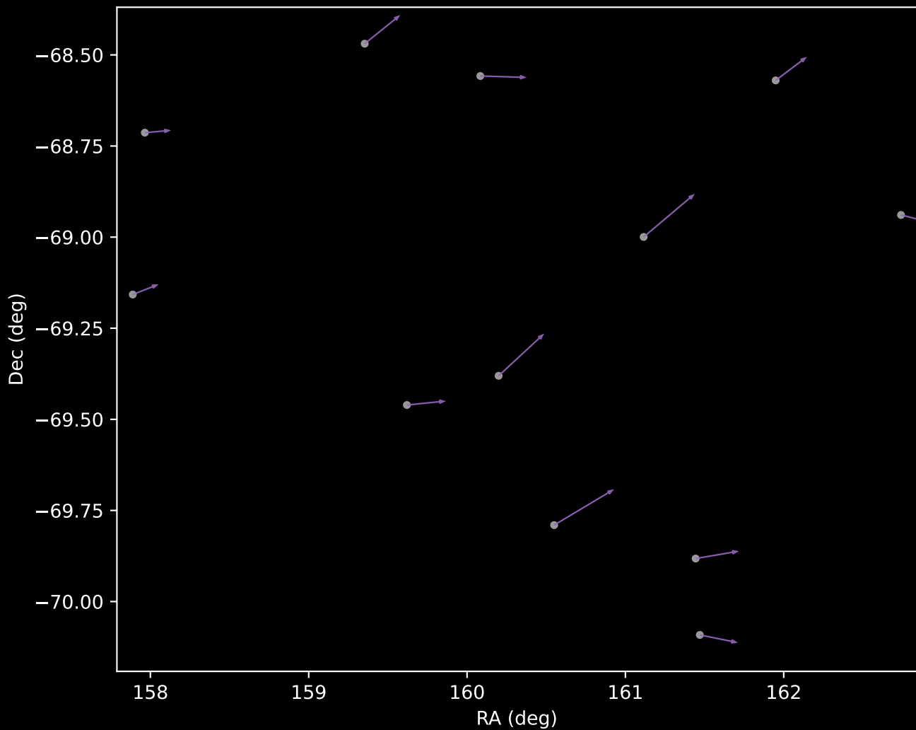
GALAH DR4 Cluster 8 Proper Motion Vectors (n=12)
