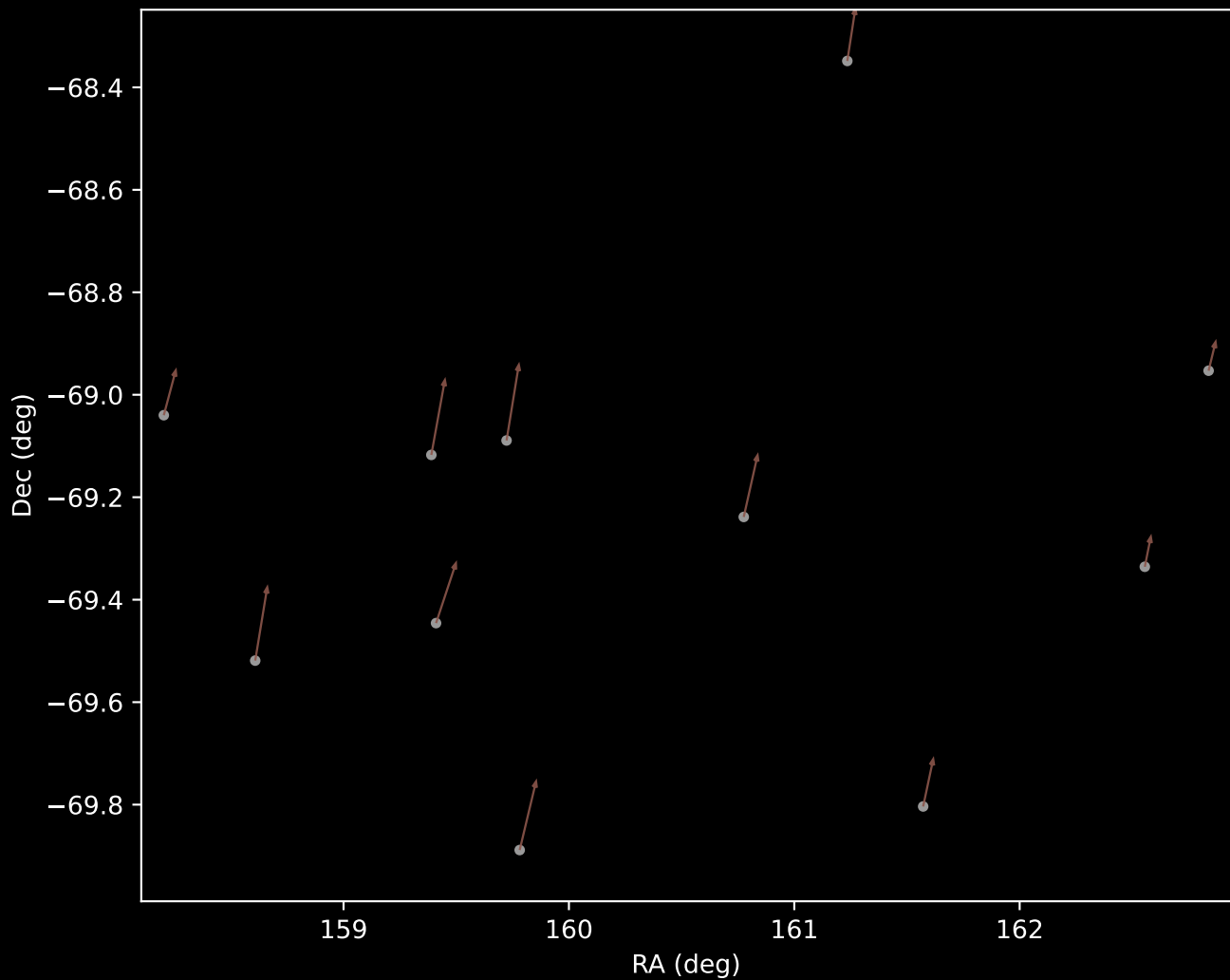
GALAH DR4 Cluster 10 Proper Motion Vectors (n=11)
