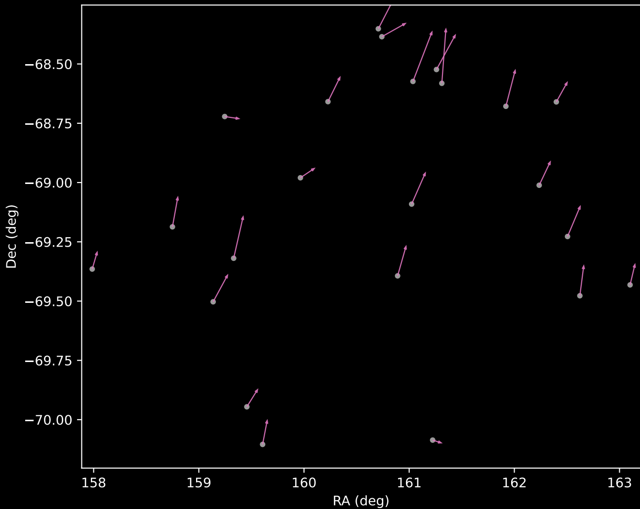
GALAH DR4 Cluster 12 Proper Motion Vectors (n=23)
