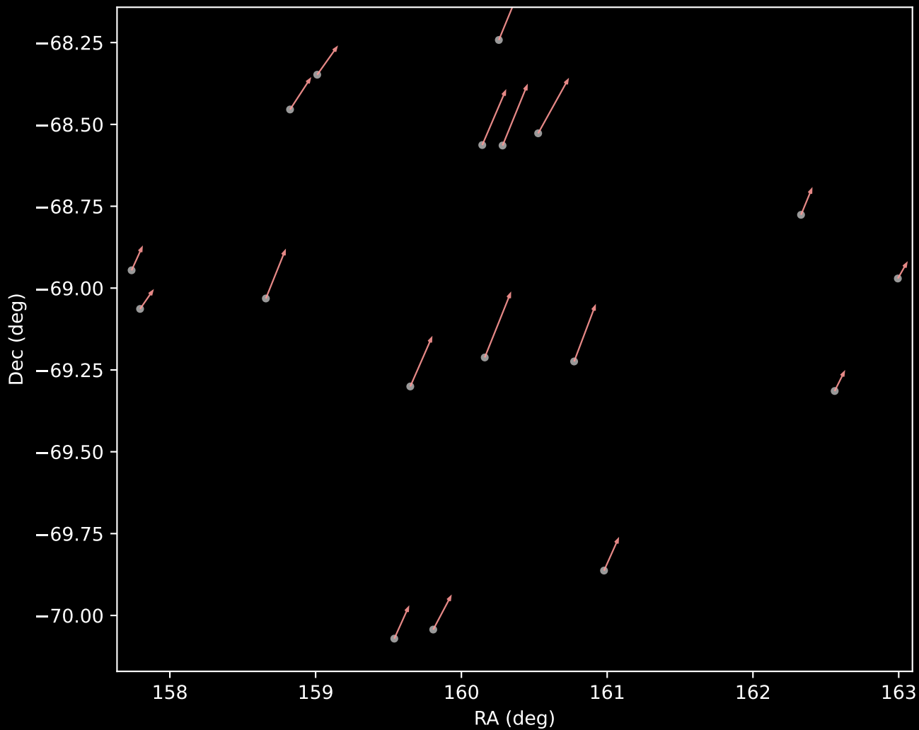
GALAH DR4 Cluster 7 Proper Motion Vectors (n=18)
